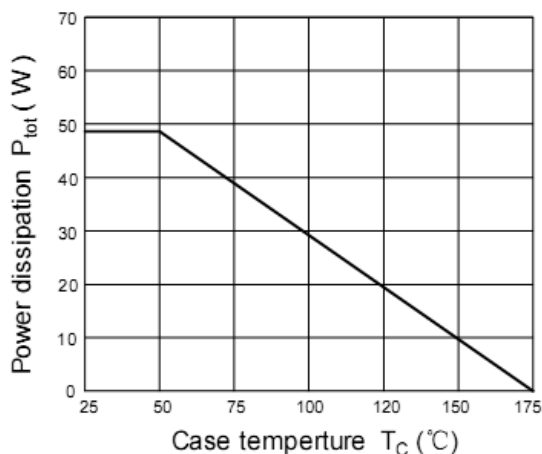
Figure 4 Power Derating
