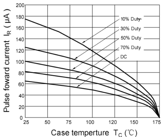
Figure 3 Current Derating
