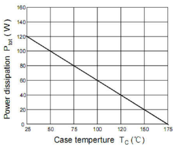
Figure 4. Power Derating
