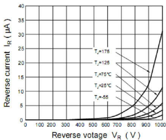
Figure 2. Reverse Characteristics
