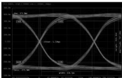
Fig.5HDMI2.0Mask at 6.0Gbps
