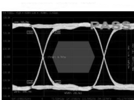
Fig.3 HDMI 1.4 Mask at 3.4 Gbps
