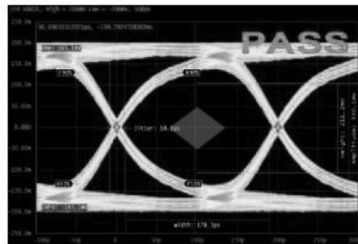
Fig.4 USB 3.0 Mask at 5.0 Gbps
