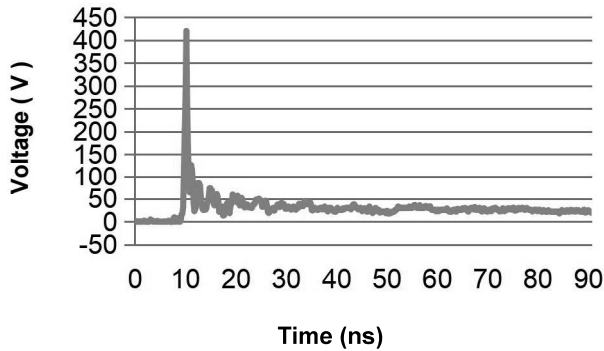
Fig.1 Typical ESD Response (IEC 61000-4-2, 8kV contact discharg)
