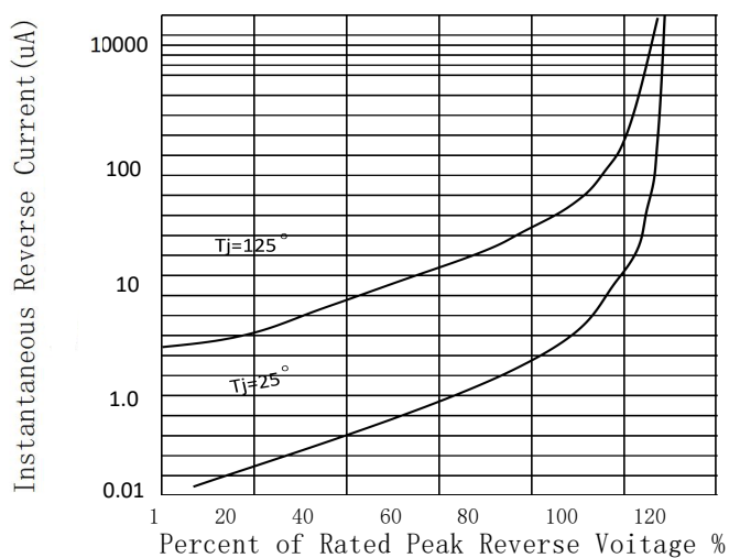
Fig. 3-Typical Reverse Characteristics
