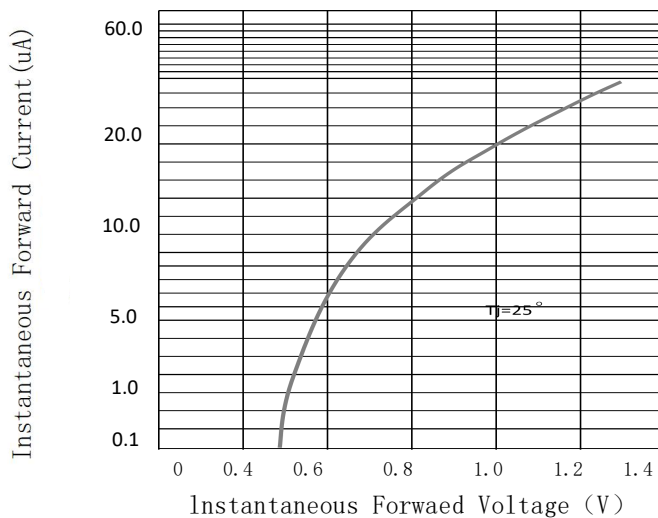
Fig.4-Typical Forwaed Characteristics
