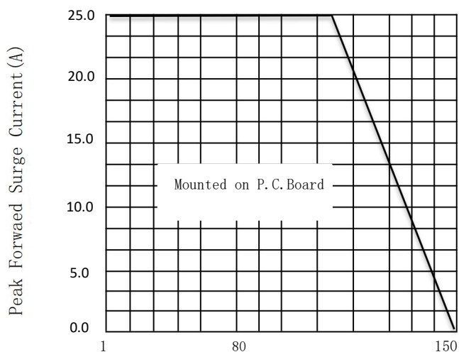
Fig. 1-forwardCurrent derating Curve
