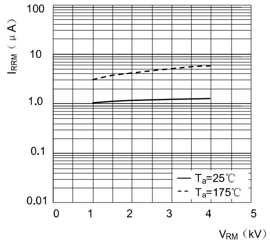
Reverse Characteristics
