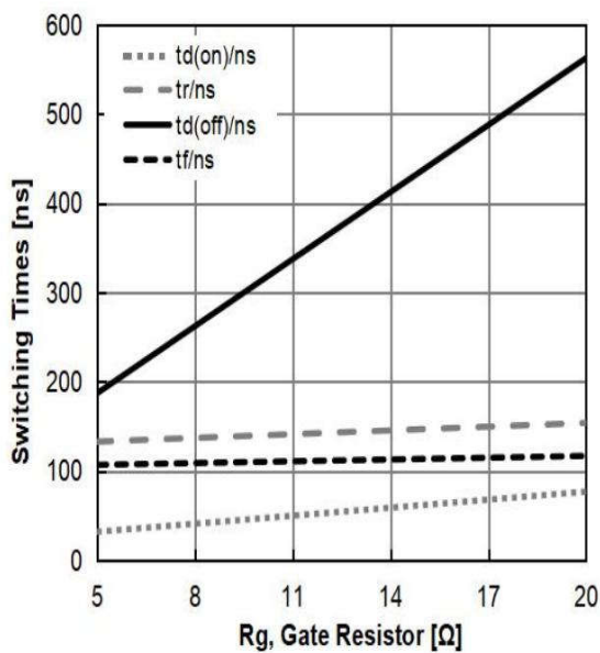
Figure 9: Typical Switching Times vs. Gate Resistor ( T_J=25^\circ\text{C} , V_{CE}=400\text{V} , V_{GE}=15/0\text{V} , I_C=75\text{A} )
