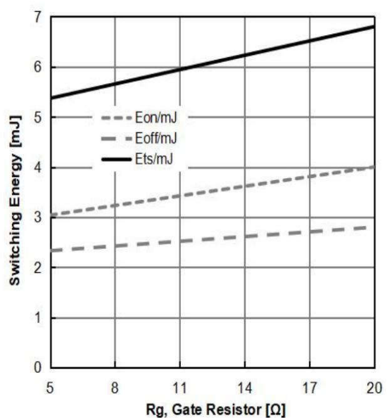
Figure 10: Typical Switching Energy vs. Gate Resistor ( T_J=25^\circ\text{C} , V_{CE}=400\text{V} , V_{GE}=15/0\text{V} , I_C=75\text{A} )
