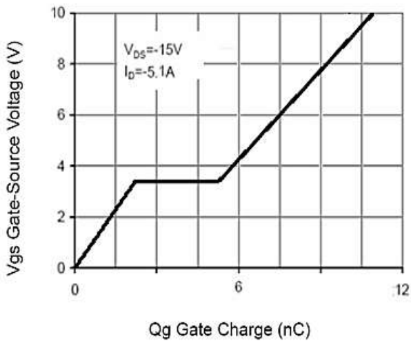
Figure 9: Gate Charge
