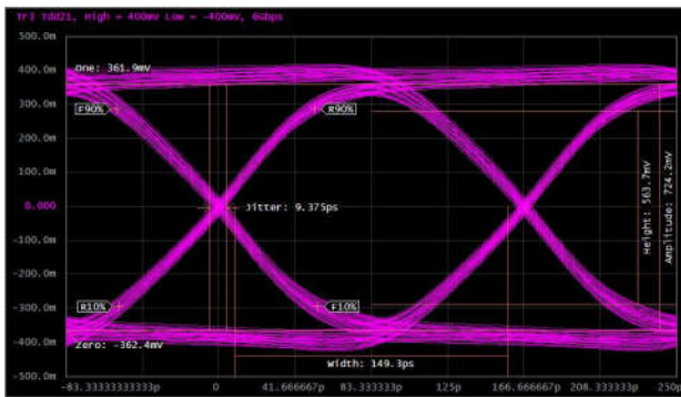
Fig.3 HDMI 2.0 Mask at 6.0 Gbps
